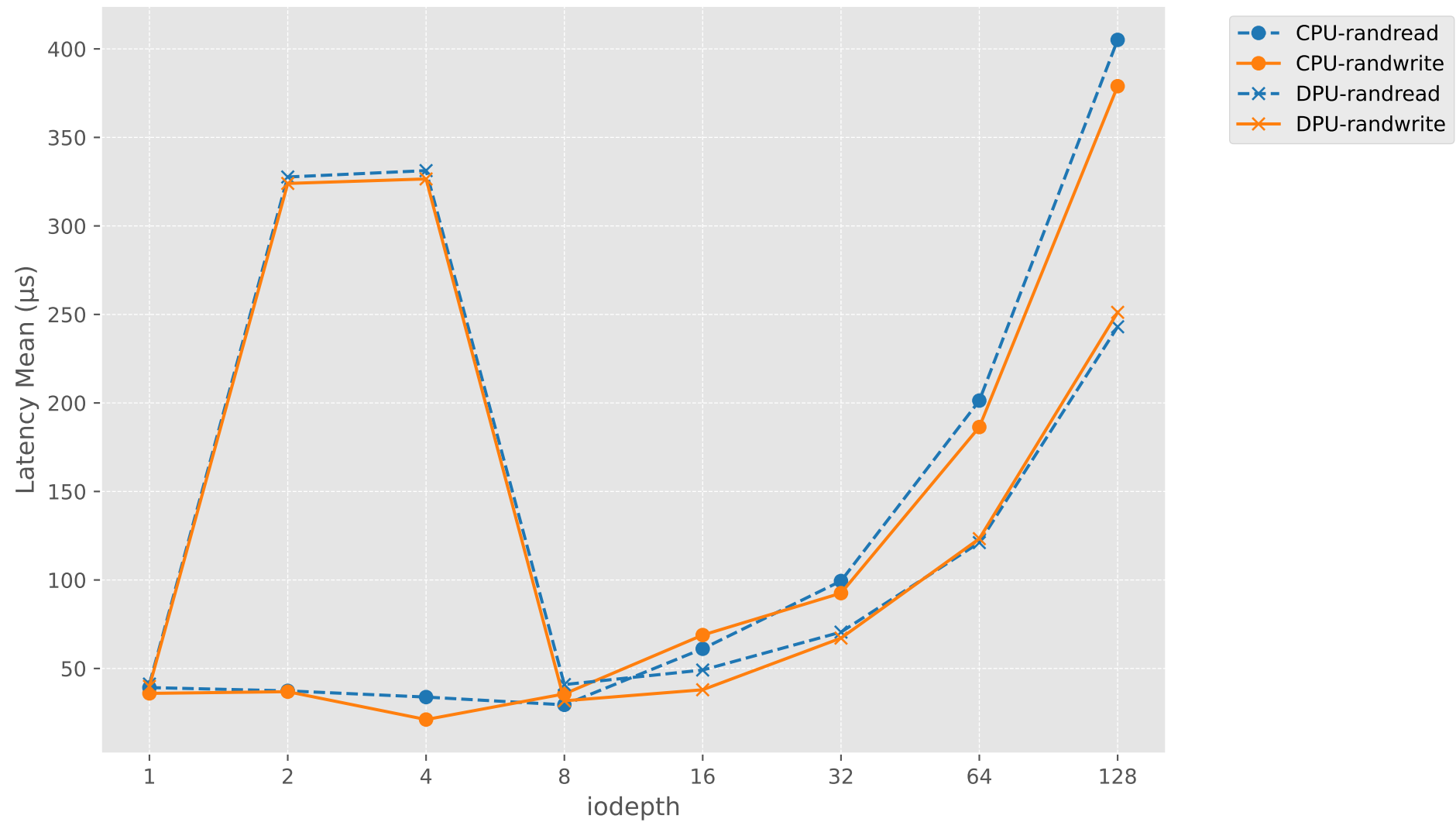
Latency Mean vs iodepth (Random)
